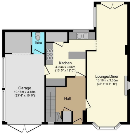
Ground Floor Floor area 82.2 sq.m. (884 sq.ft.)
